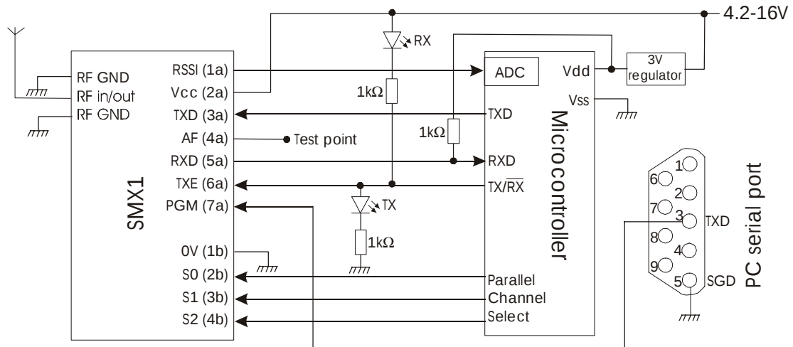
Figure 4: SMX1 interfaced to host microcontroller and serial port for configuration
