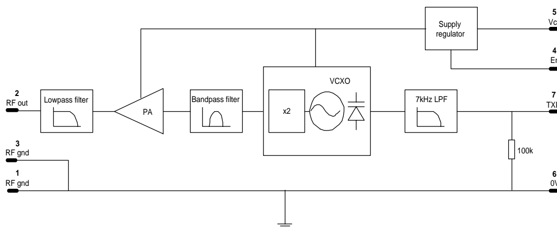
Fig.1: TX1 block diagram
