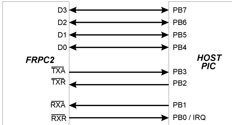
figure 16: RPC2 to PIC - \mu C interface
