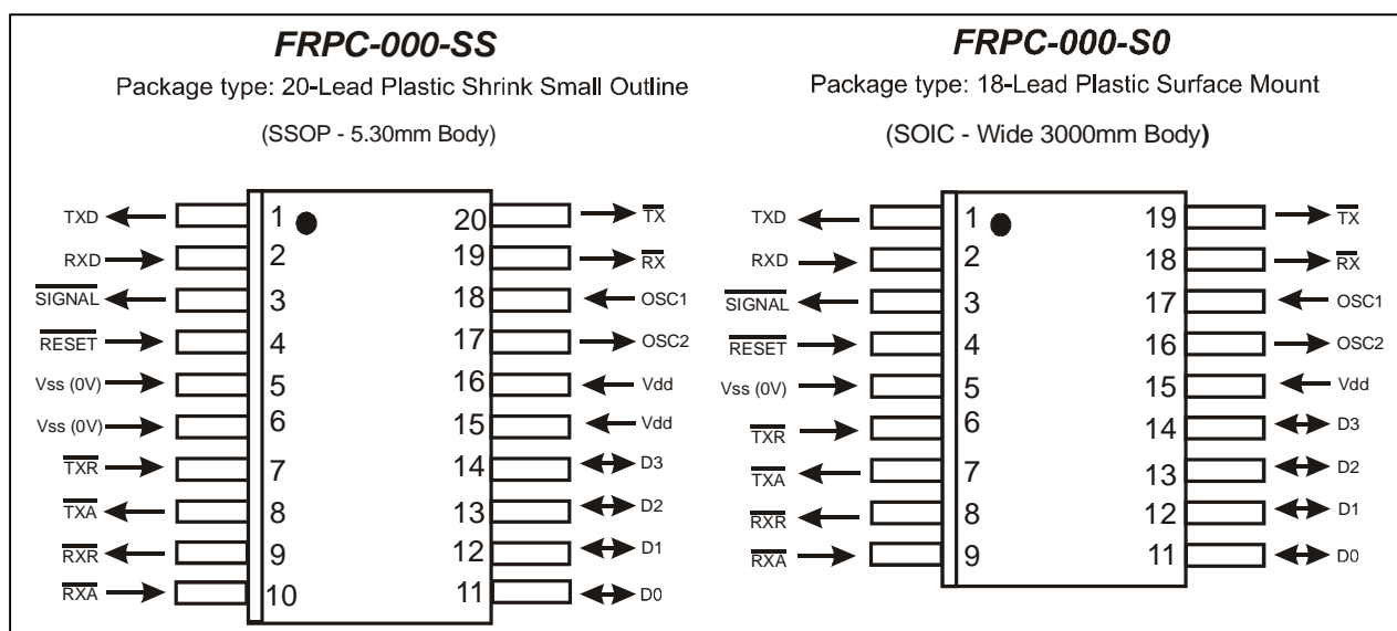
figure 18: FRPC-000-SS & FRPC-000-S0
